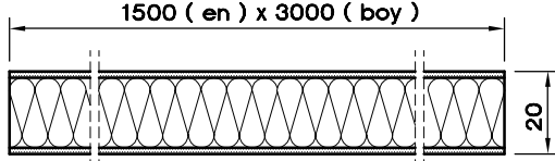
SANDWICH PANEL (20)
