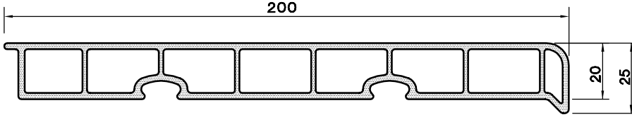
PARAPET PR. ( 200 x 25 ) 1399.337
