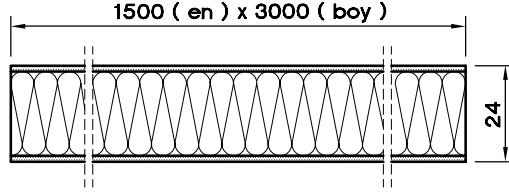
SANDWICH PANEL (24) H999.124
