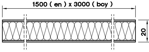
SANDWICH PANEL-20 S999.120
