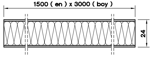
SANDWICH PANEL-24 S999.124
