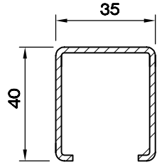
U DESTEK SACI 35x40 (2.0) 5170.512
