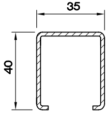
U DESTEK SACI 35x40 (1.5) 5170.511
