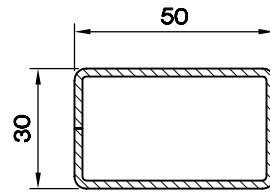
KUTU PR.(30X50-2.0) 5399.222
