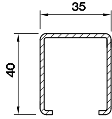
U DESTEK SAÇI 35x40 (1.5) 5170.511
