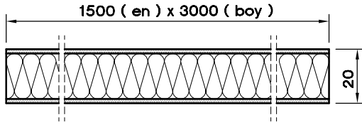
SANDWICH PANEL (20) H999.120
