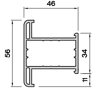
KEPENK ORTAKAYIT-56 PR. 11PK3560000000000
