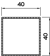
AL. KUTU 40x40-1.2 61PK1100000000000
