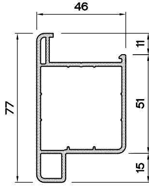
KEPENK BİNİLİ KANAT-77 PR. 11PK4770000000000
