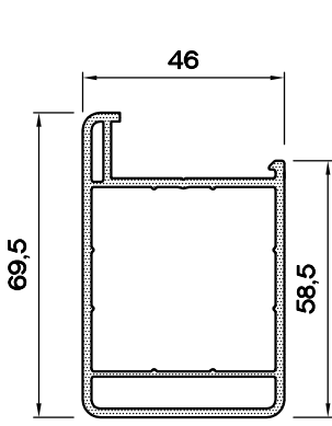
KEPENK KANAT-69 PR. 11PK2690000000000
