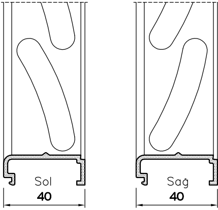
DELİKLİ SABİT LAMEL ÇİTASI TAKIMI 12PK1010000000000
