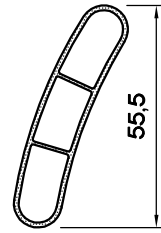
KEPENK SABİT LAMEL PR. 12PK1030000000000
